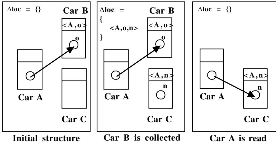
Figure 2: Illustration of algorithm handling movement of objects
